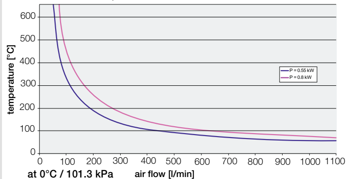
temperature – air flow characteristics
